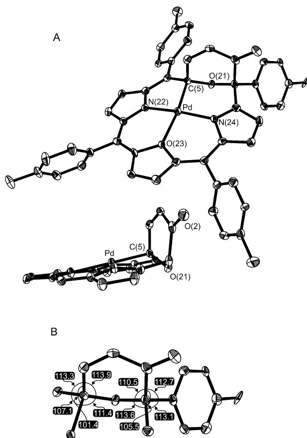
Figure 4. The X-ray molecular structure of 4 . A) Overall geometry of the molecule and the projection emphasizing the perpendicular orientation of the 3-pyrone ring enforced by coordination [Pd(1)–C(5) 1.995(3), Pd(1)–N(22) 1.924(2), Pd(1)–O(23) 2.107(2), and Pd(1)–N(24) 1.979(2)]. B) Selected bond angles around two sp 3 carbon atoms C(1) and C(5)]. [17]
